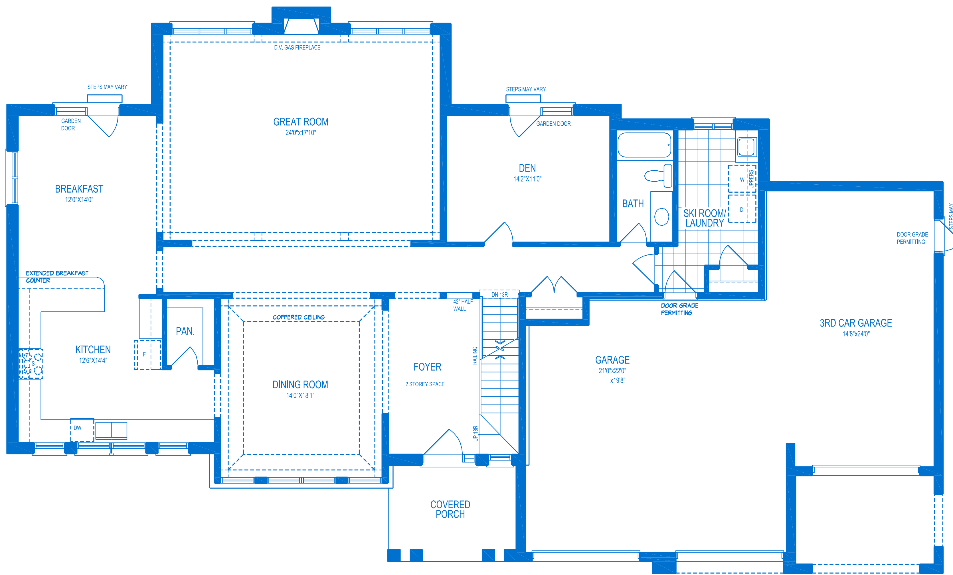
MAIN FLOOR PLAN 'C'
