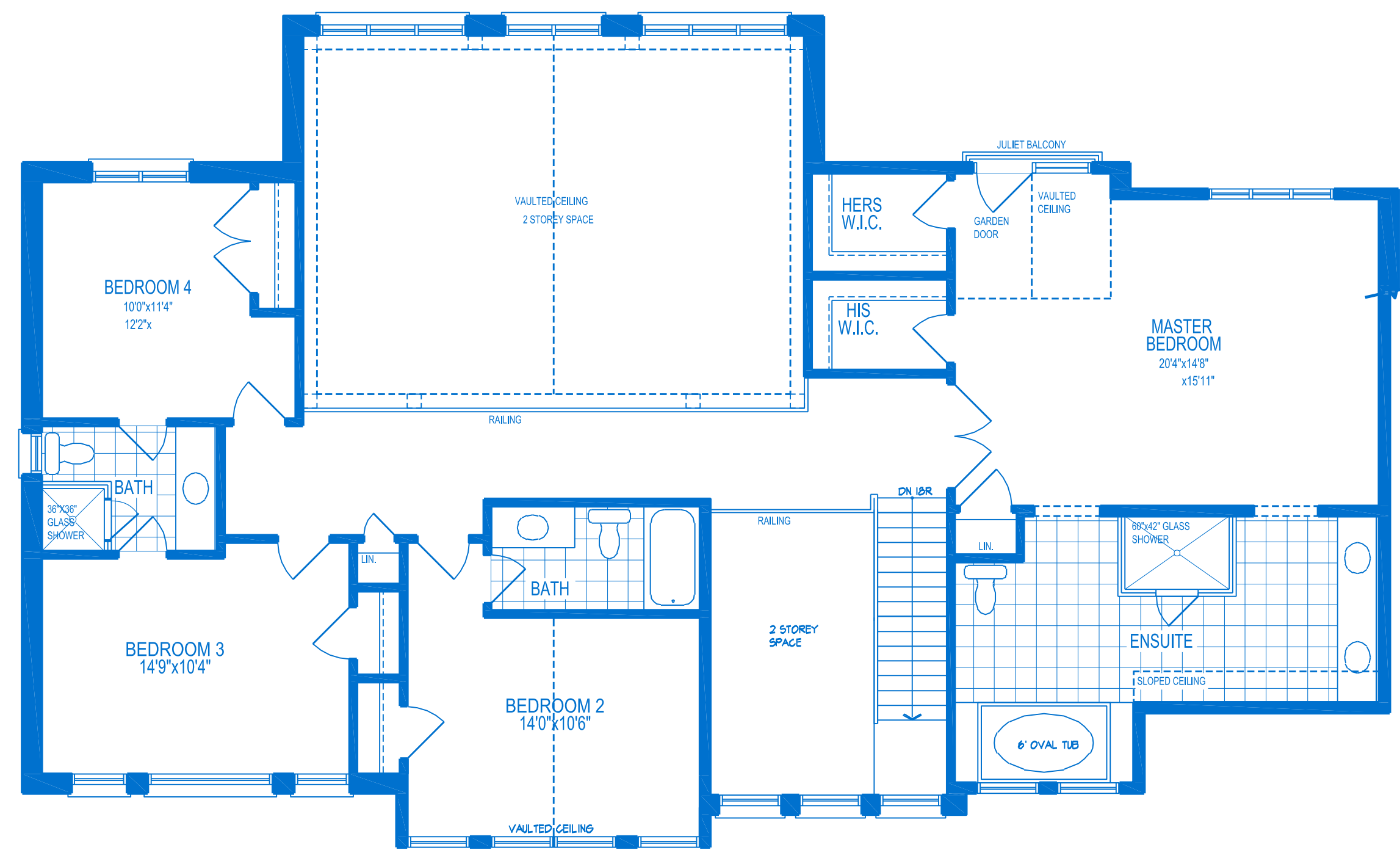
UPPER FLOOR PLAN 'C'
