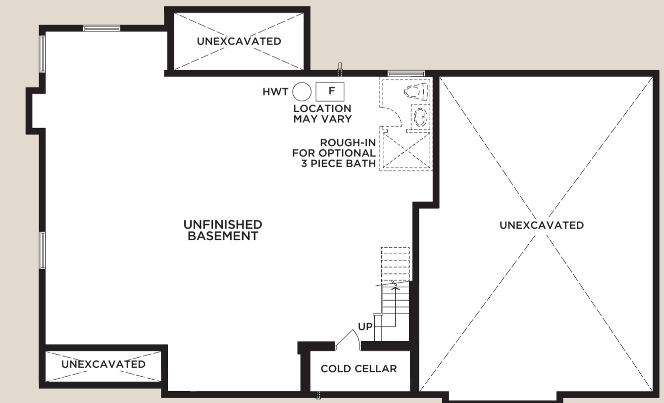
Basement Level Elev A
