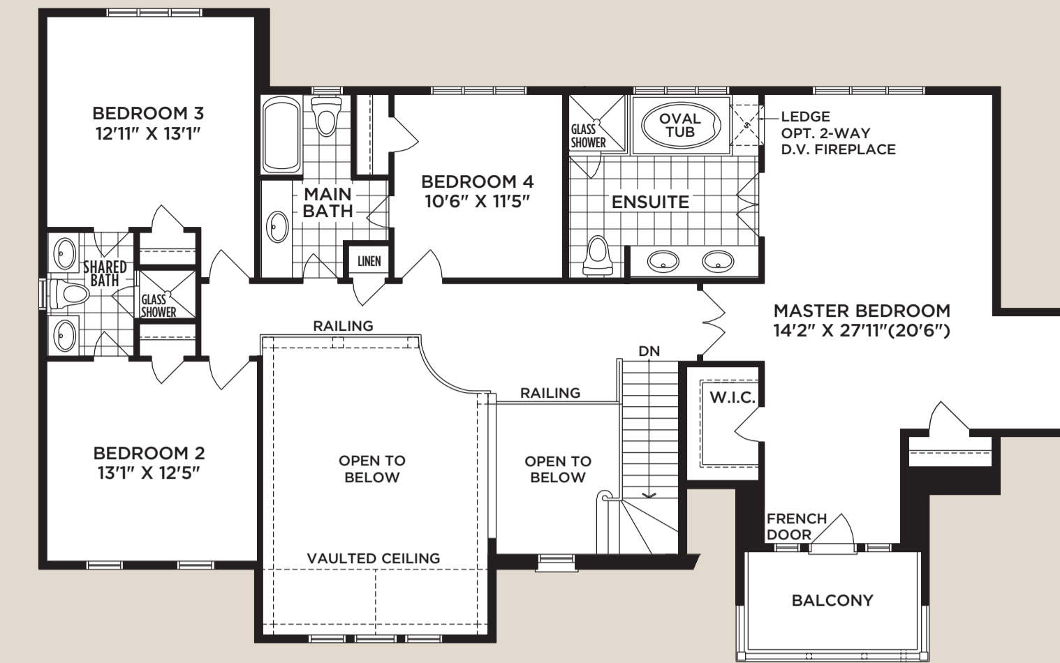
Upper Level Elev A
